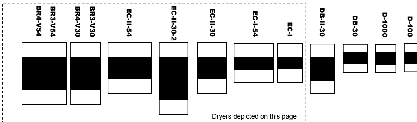
Dryer foot print comparison chart, shown to scale
